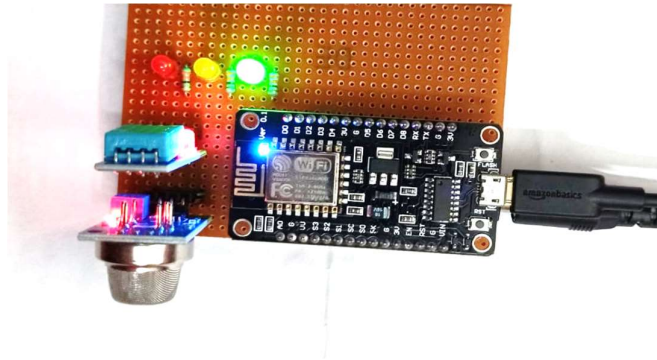
Fig: 5.8 Setup for Experiment 4
