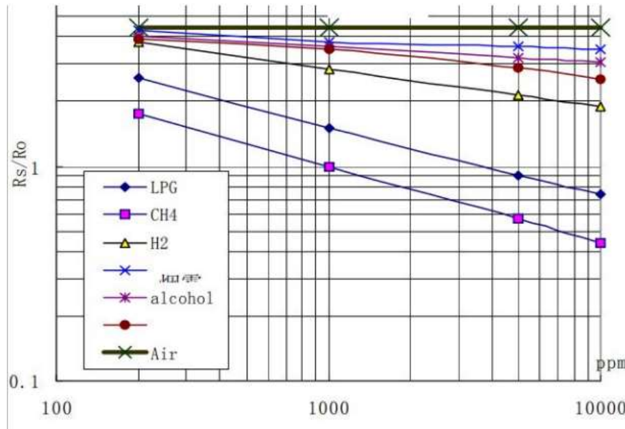
Fig. 4.2 (Graph representing ratio vs ppm variations)
